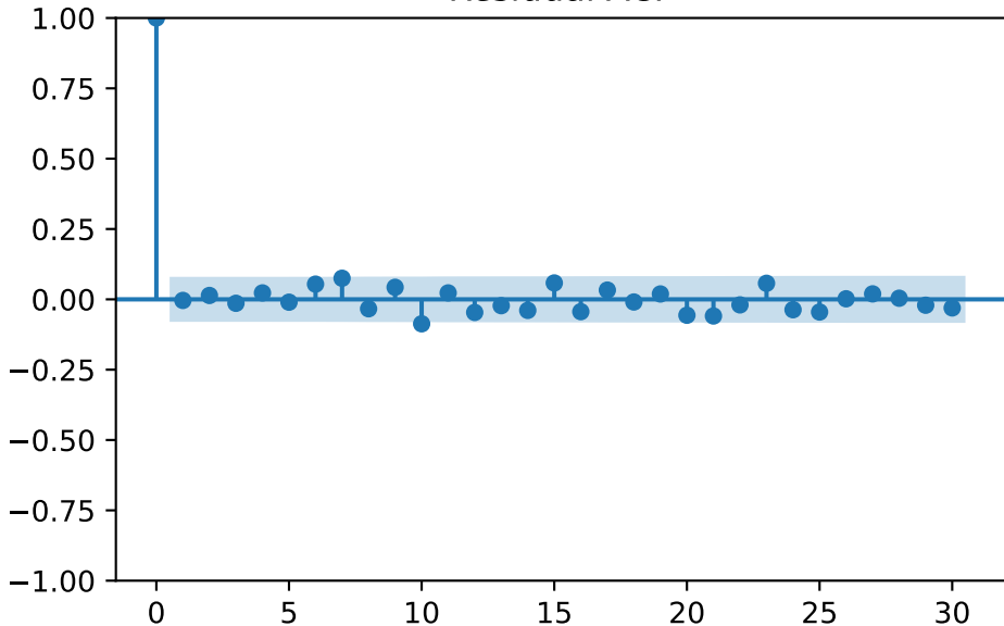
Residual ACF
