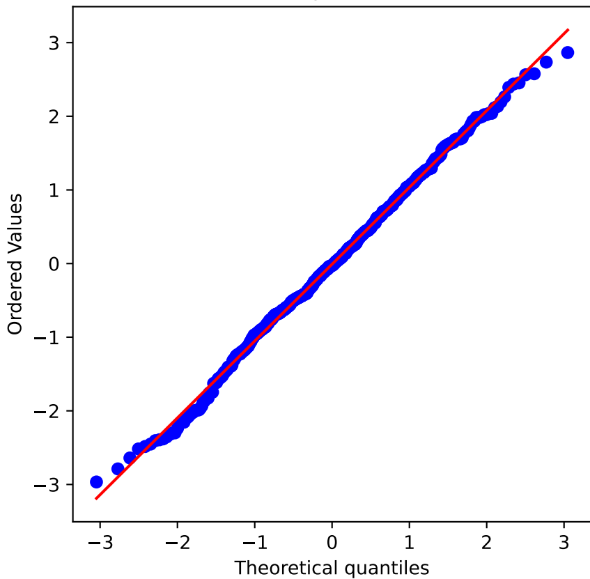
Normal Q-Q plot of residuals
