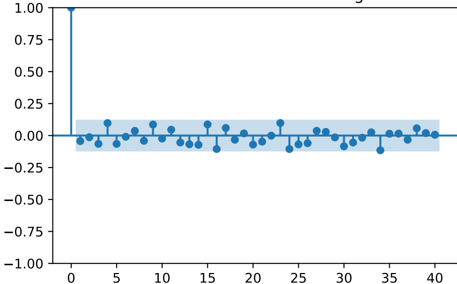
PACF after first differencing
