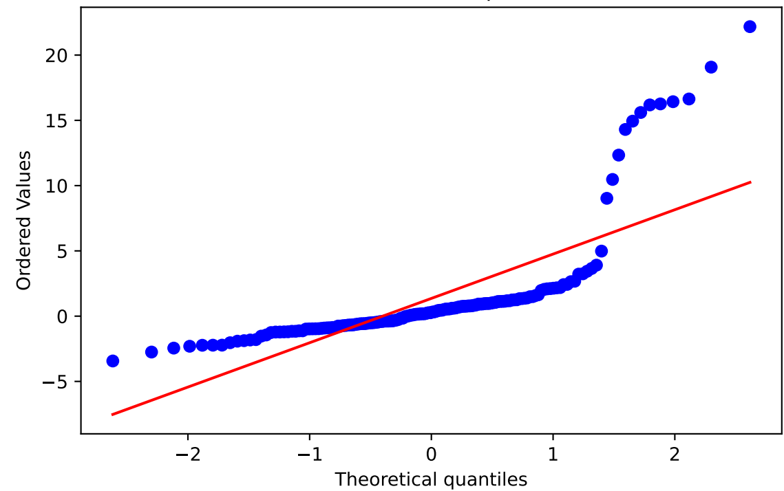
Residual Q-Q plot
