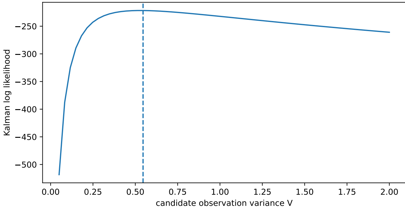
Grid likelihood for observation noise variance
