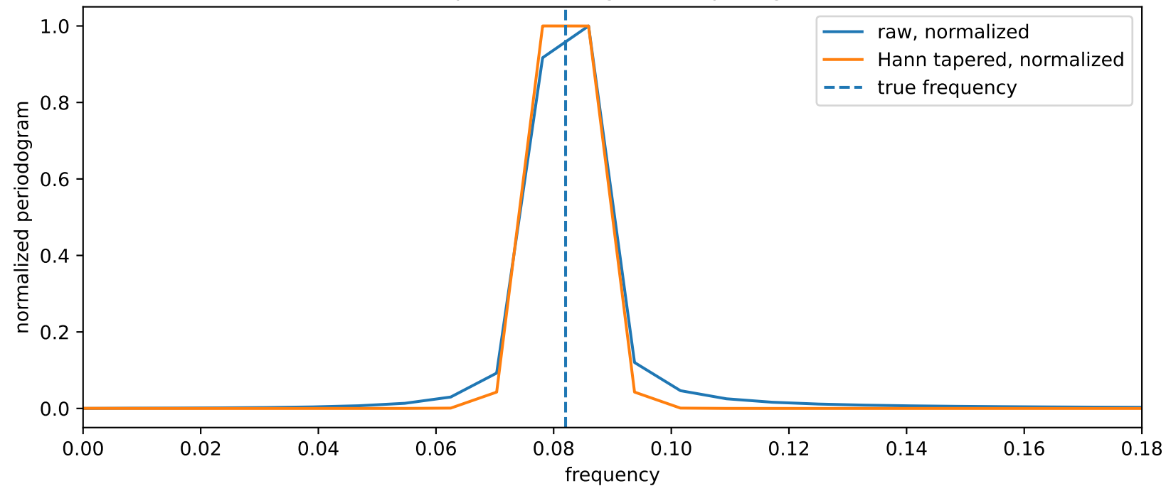
Spectral leakage and tapering
