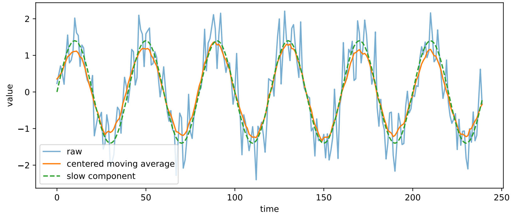
Low-pass smoothing with a moving-average filter
