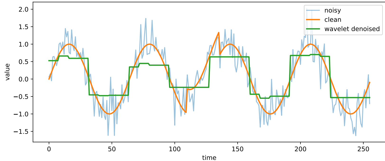
Wavelet denoising with soft thresholding
