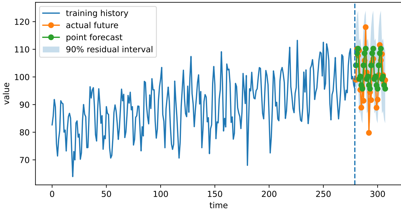
Residual-based forecast interval
