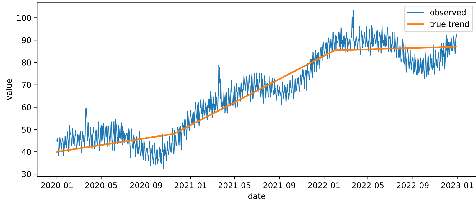
Synthetic additive forecasting data
