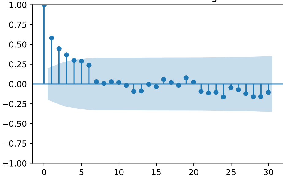
ACF of test errors for ridge
