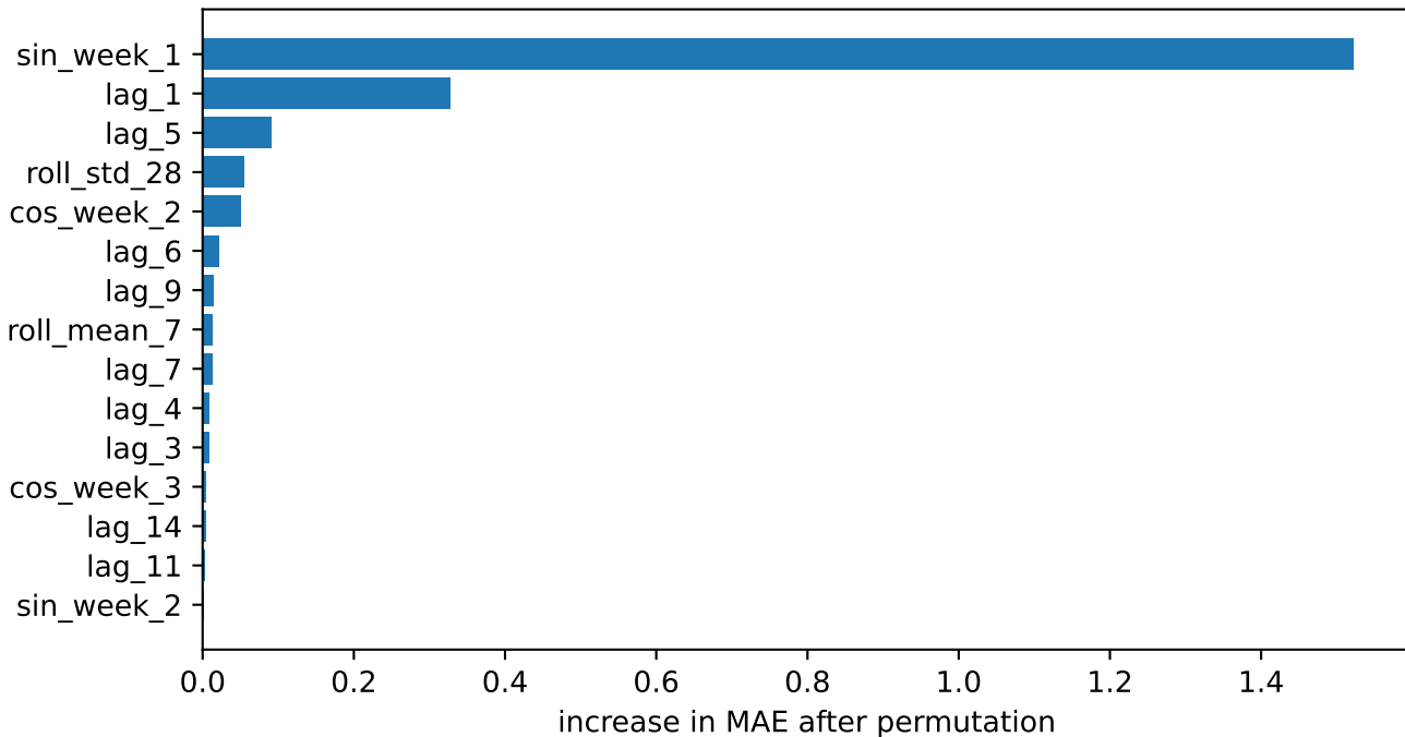
Permutation importance, top features
