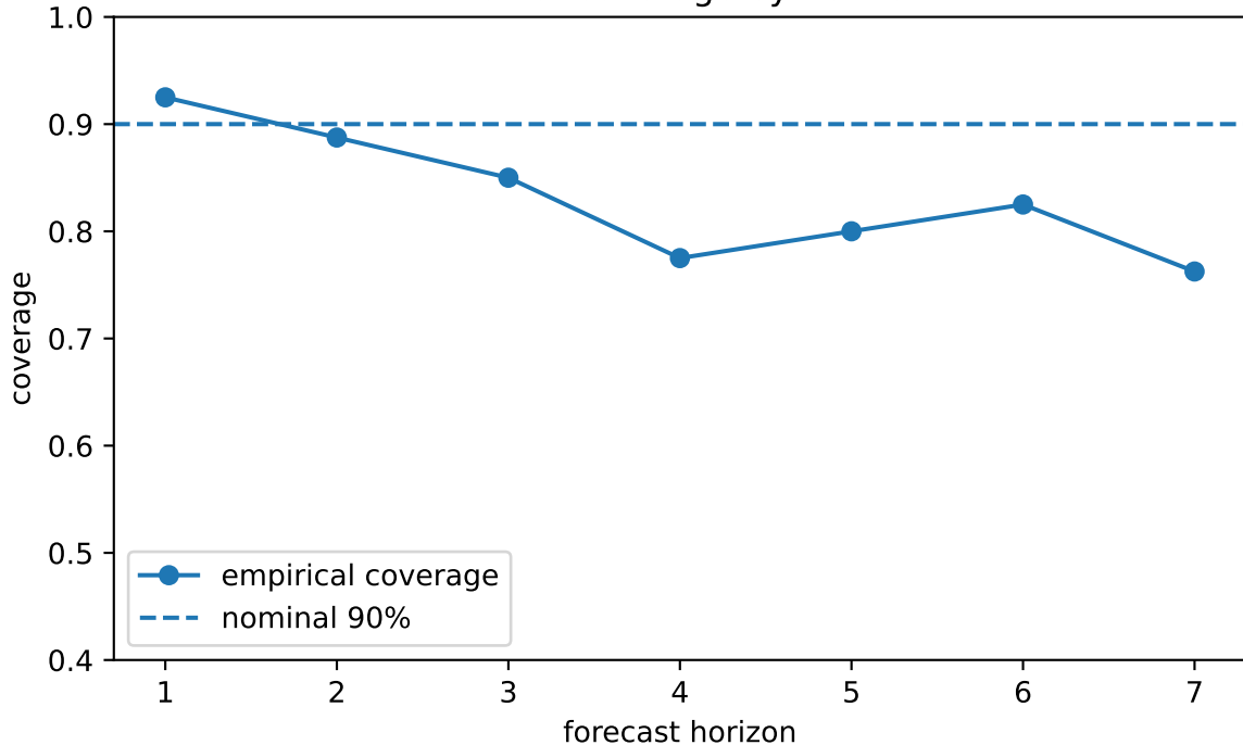
Interval coverage by horizon
