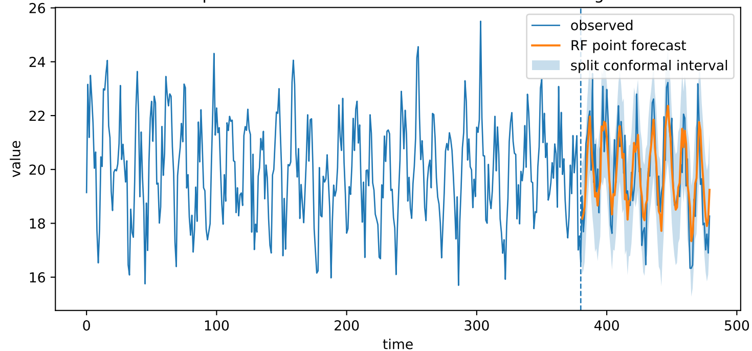
Split conformal interval for time-series forecasting
