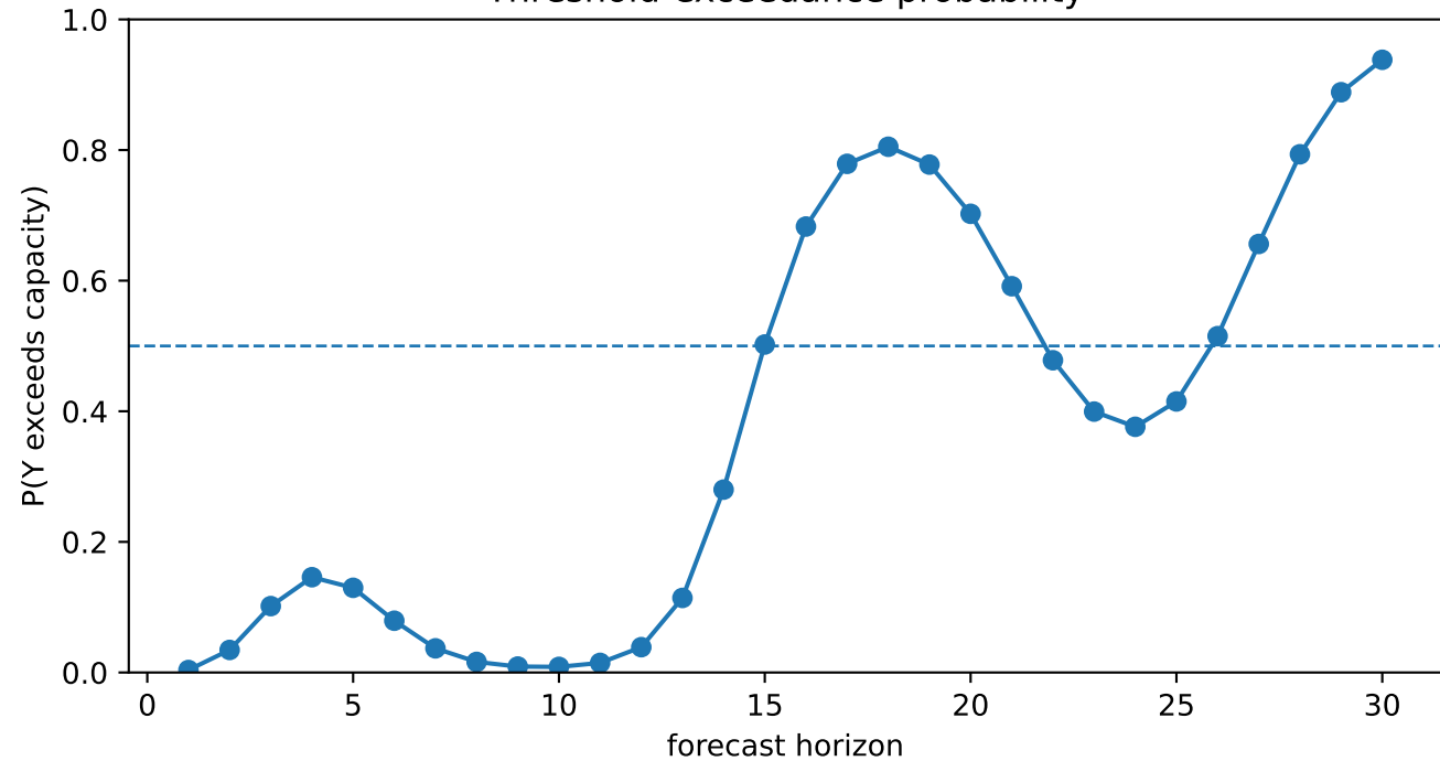
Threshold-exceedance probability
