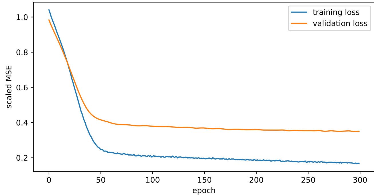
MLP training history
