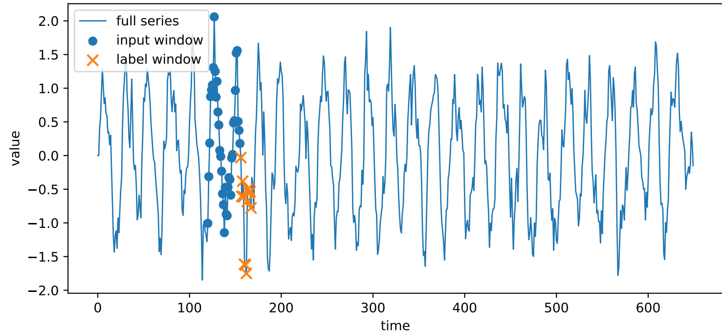
A supervised example produced from a time series
