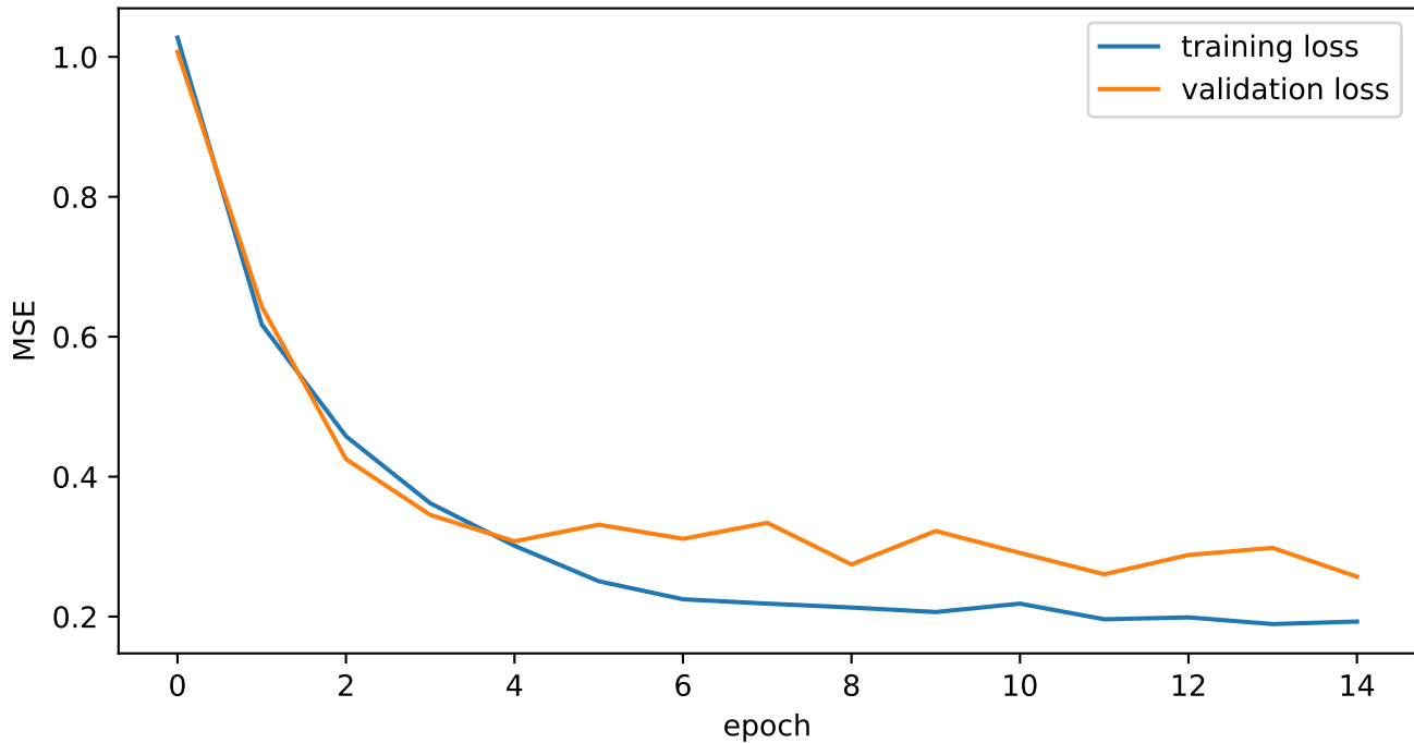
TCN training curve
