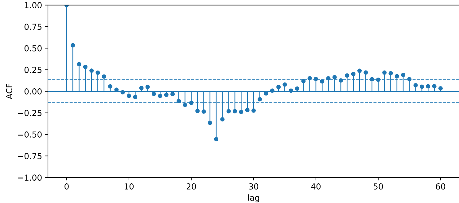
ACF of seasonal difference
