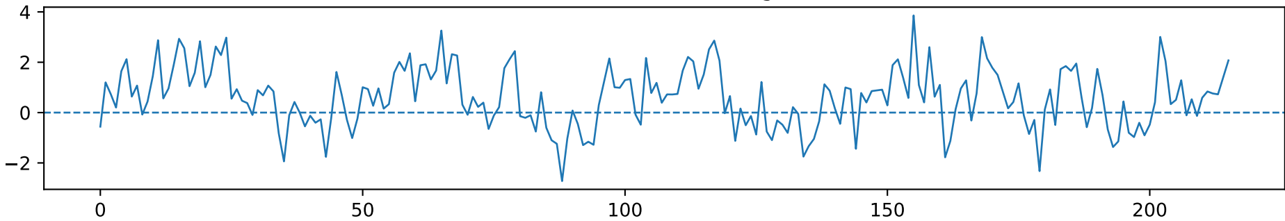
First difference followed by seasonal difference
