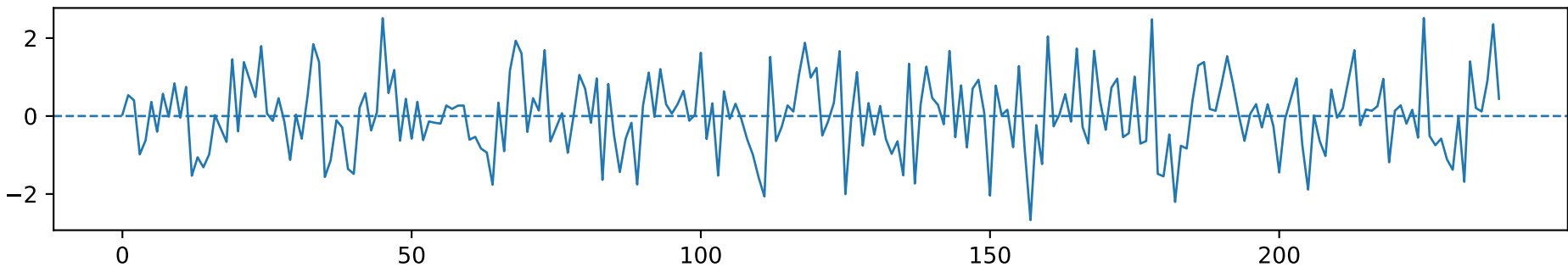
Seasonal difference, lag=24
