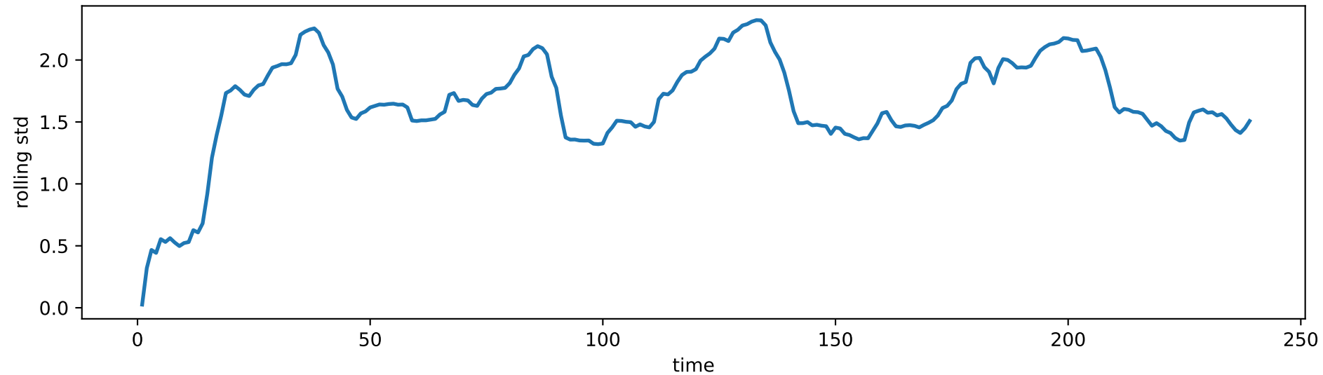
Rolling standard deviation
