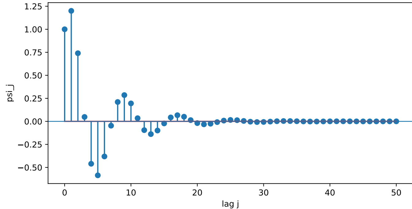
Impulse-response coefficients for AR(2)
