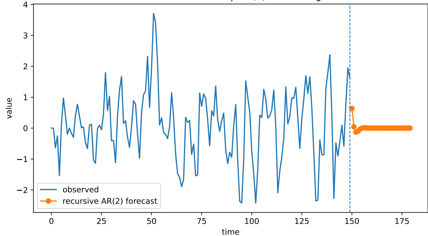
Recursive multi-step AR(2) forecasting
