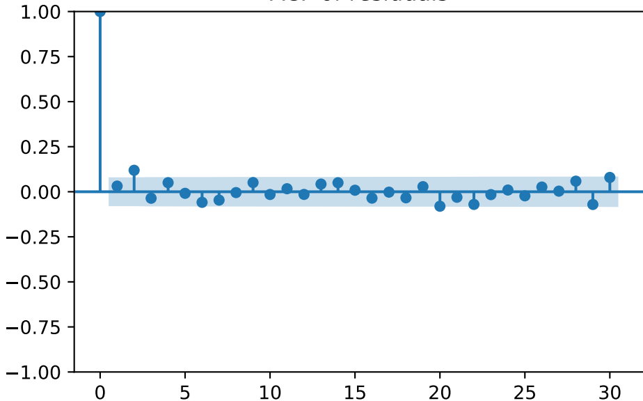
ACF of residuals
