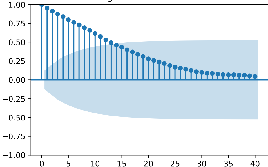
ACF of original random walk with drift
