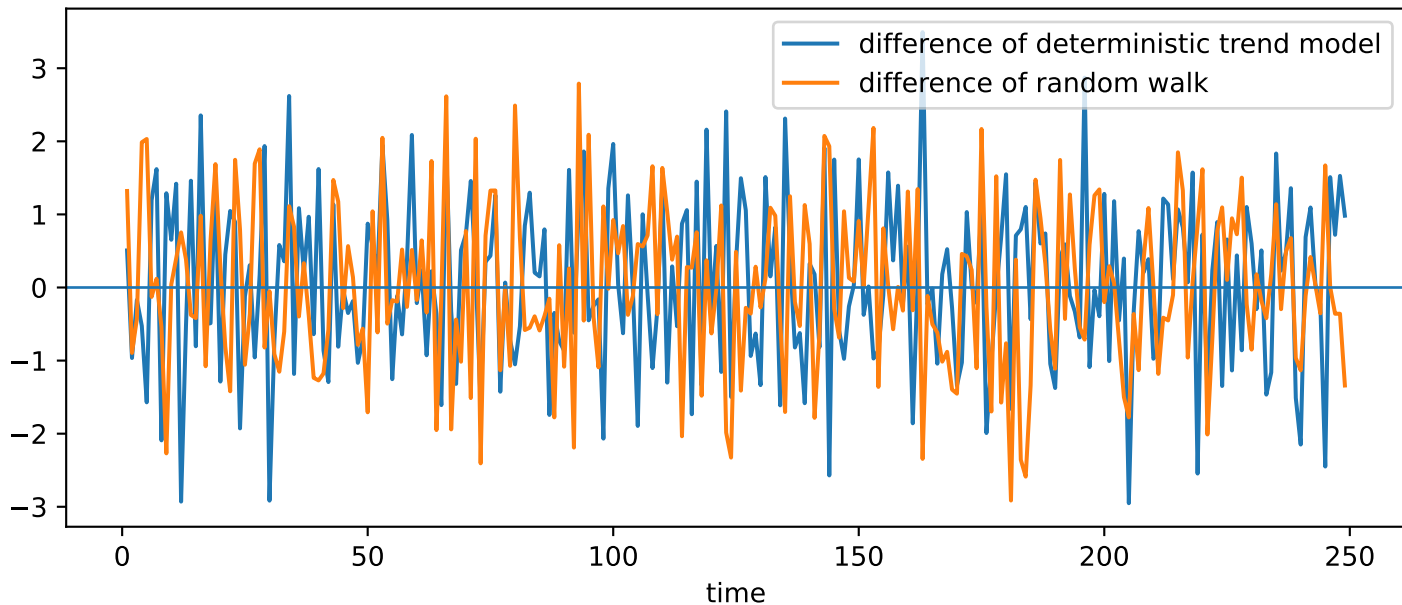
First differences
