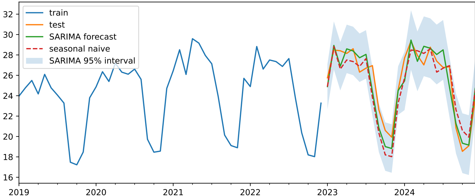
SARIMA forecast versus seasonal naive baseline
