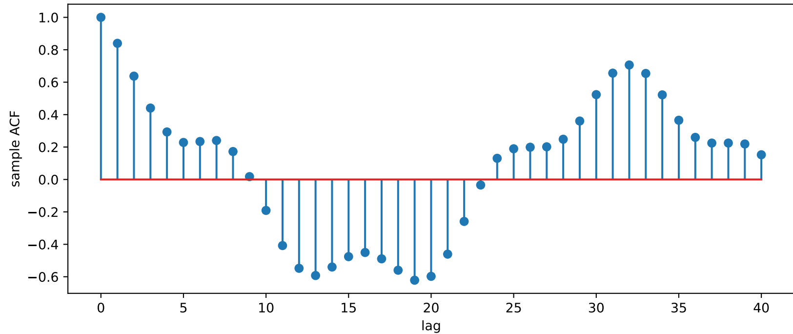
Sample ACF
