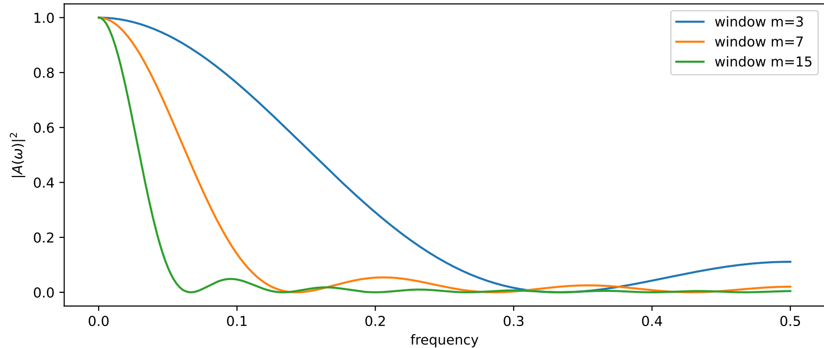
Frequency response of simple moving-average filters
