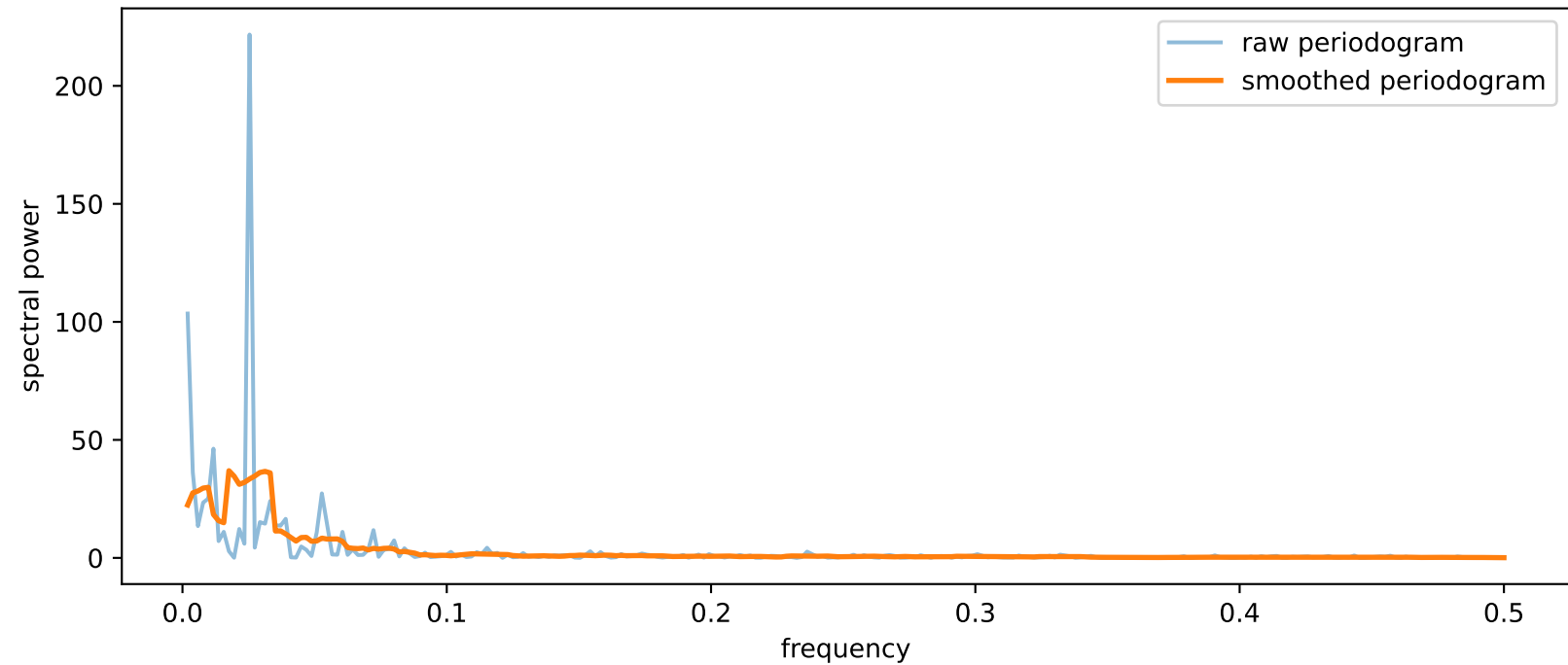
Raw versus smoothed periodogram
