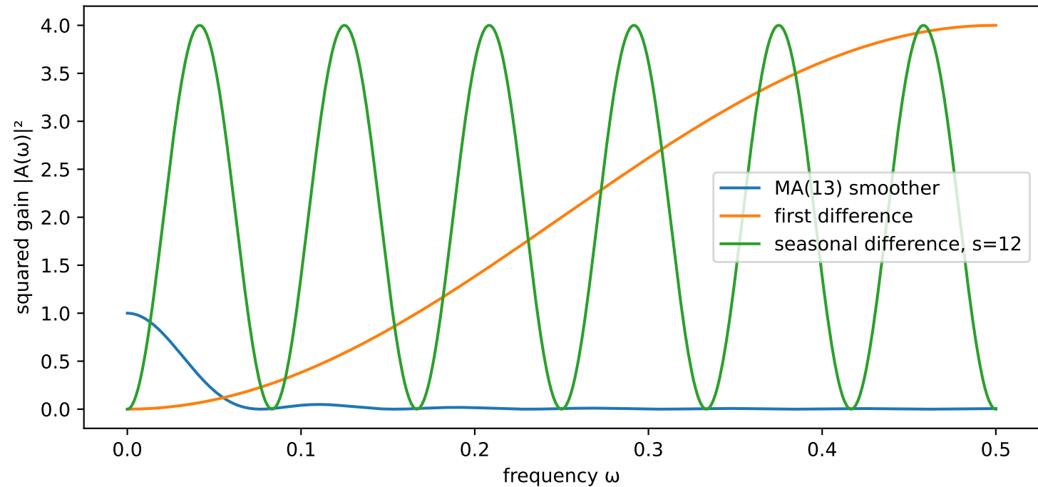
Frequency responses of three filters
