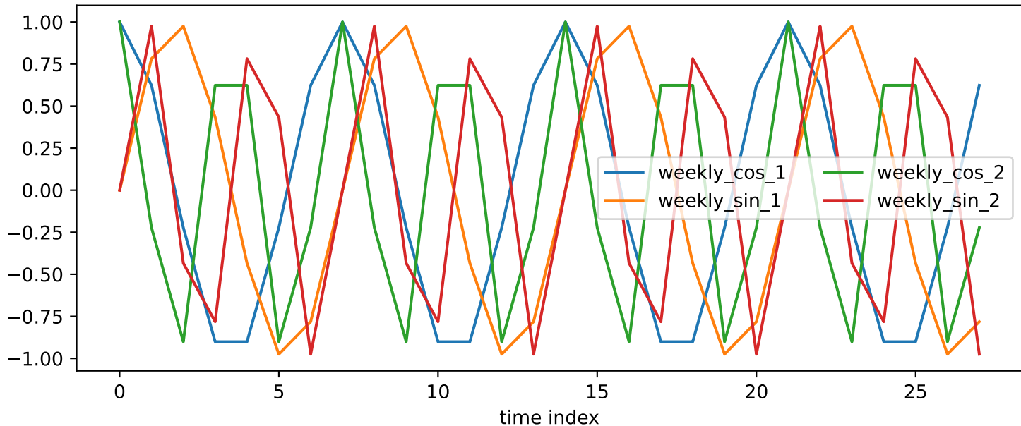
First weekly Fourier basis functions
