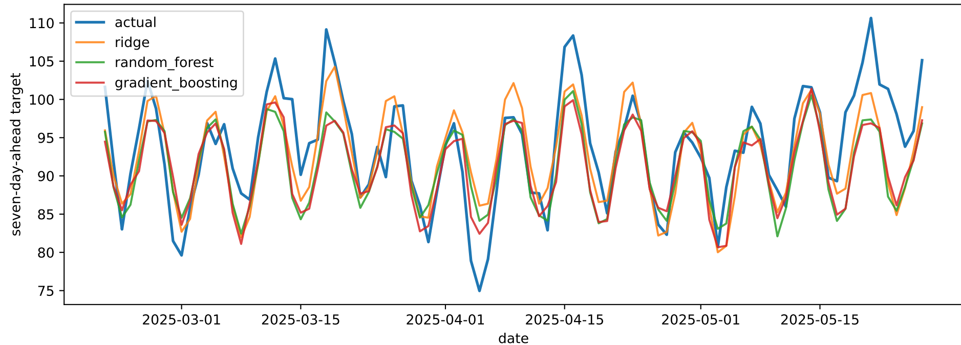
Feature-based ML forecasts on chronological test period
