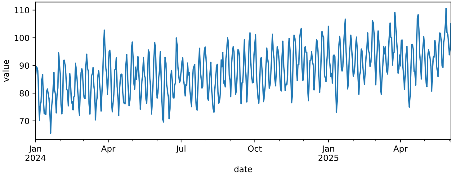
Synthetic series with trend, seasonality, and dependence
