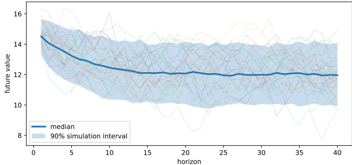
Simulated future paths
