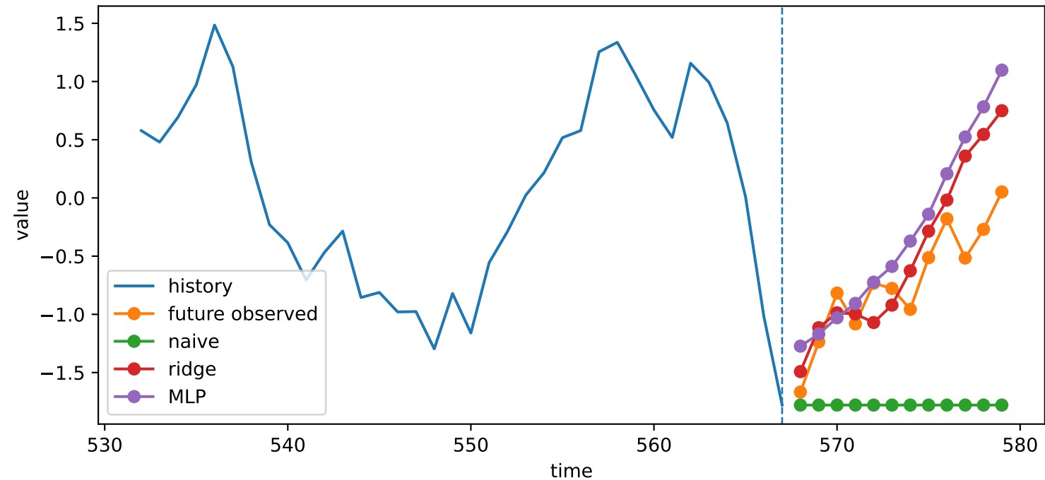
One multi-step forecast from a held-out test window
