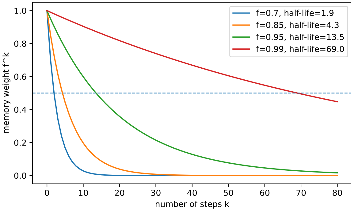
Direct memory decay controlled by the forget gate
