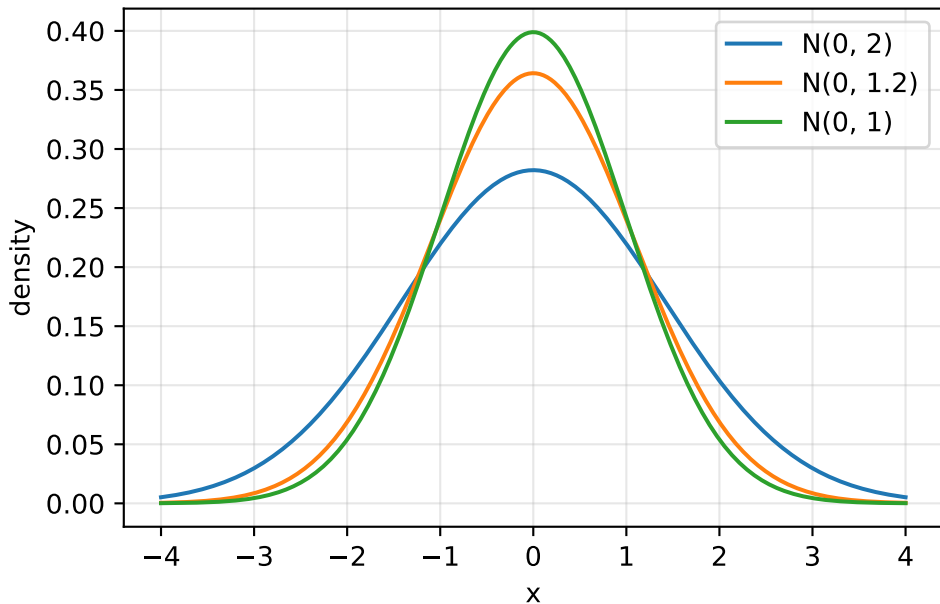
Normal densities approaching N(0, 1)
