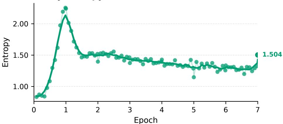
Policy Entropy [0.8335, 2.255]
