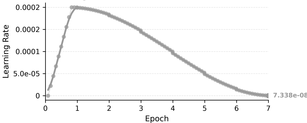
Learning Rate [0, 0.0002]
