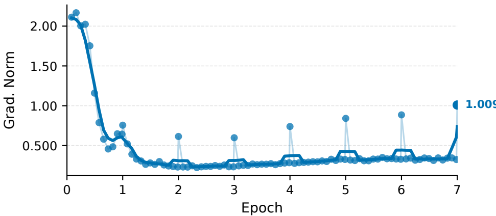
Gradient Norm [0.2226, 2.168]
