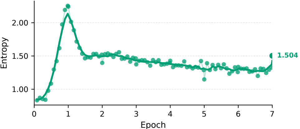
Policy Entropy [0.8335, 2.255]
