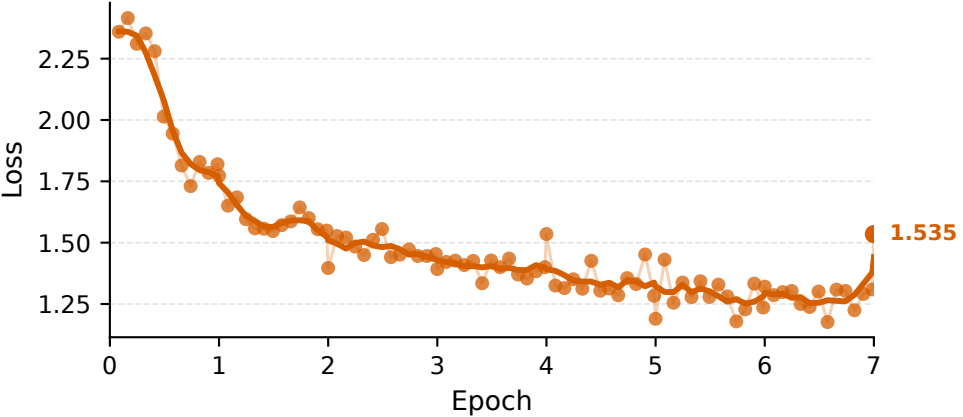
Training Loss [1.177, 2.416]
