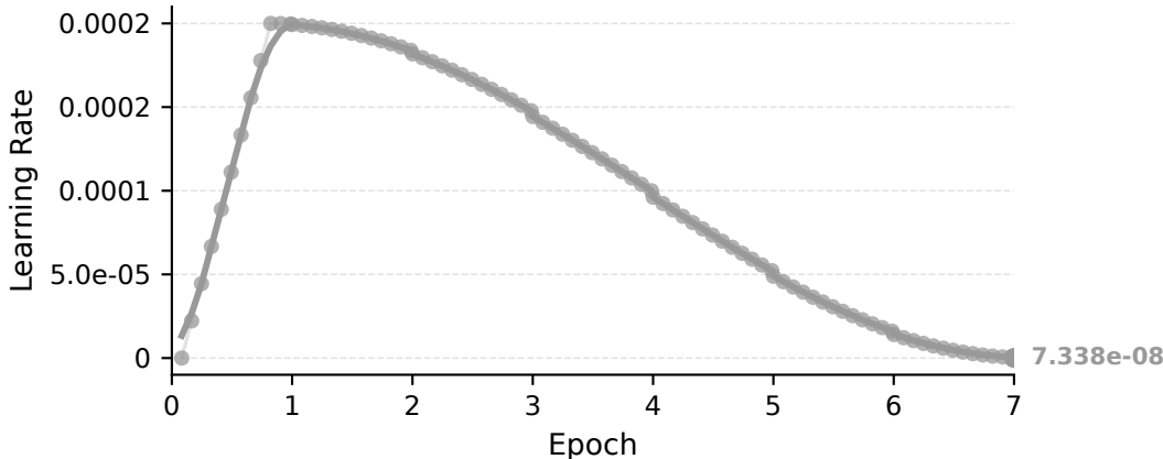
Learning Rate [0, 0.0002]
