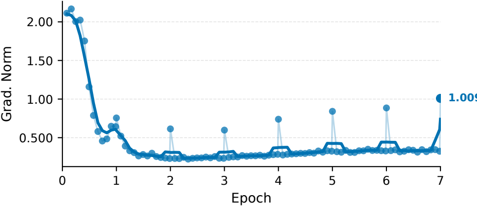
Gradient Norm [0.2226, 2.168]
