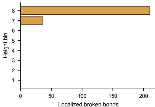
c Damage localizes near the loaded surface
