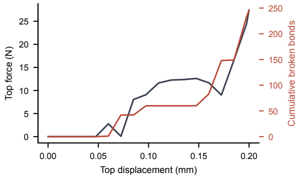
a Compression response
