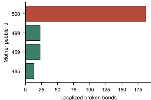
d Few pebbles initiate early breakage
