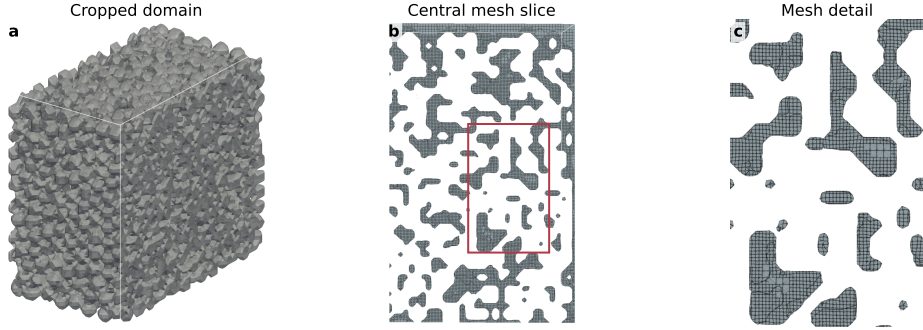
Figure 6: Cropped-domain OpenFOAM model and mesh context for the returned pressure checks. The representative N10000 peak-blockage handoff case is shown as a rendered solid-interface domain, a central mesh slice and a local mesh-detail crop. This figure documents the numerical model and mesh used for the cropped-domain pressure check; it is not experimental validation or pressure calibration for I_b .
