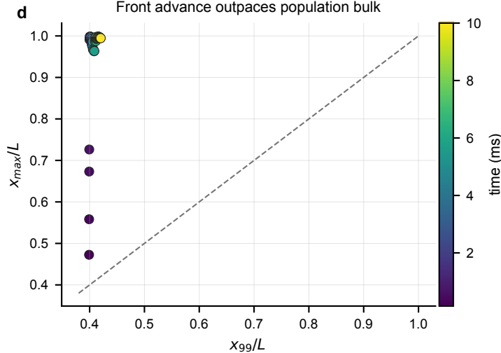
Front advance outpaces population bulk
