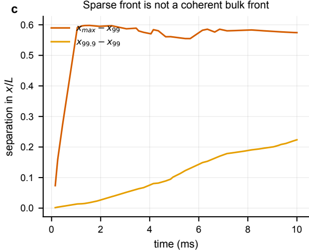
Sparse front is not a coherent bulk front
