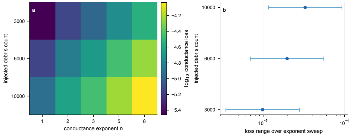
Fig. S4. conductance-exponent sensitivity for cropped peak-blockage domains. Boundary: Sensitivity of the scalar conductance response to the conductance exponent.
