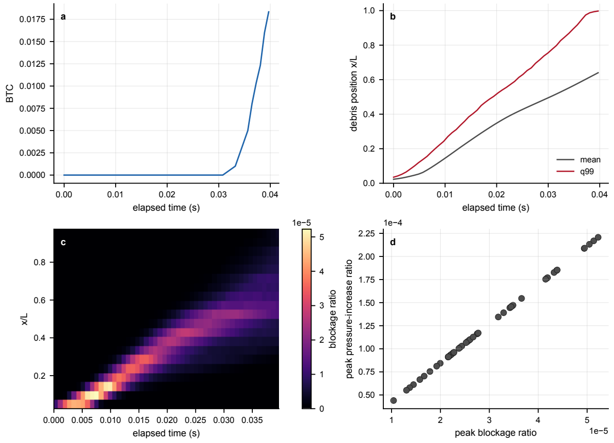
Fig. S1. time-resolved deposition and BTC for representative loading case. Boundary: Representative time-resolved support for the delayed leading-tail interpretation.
