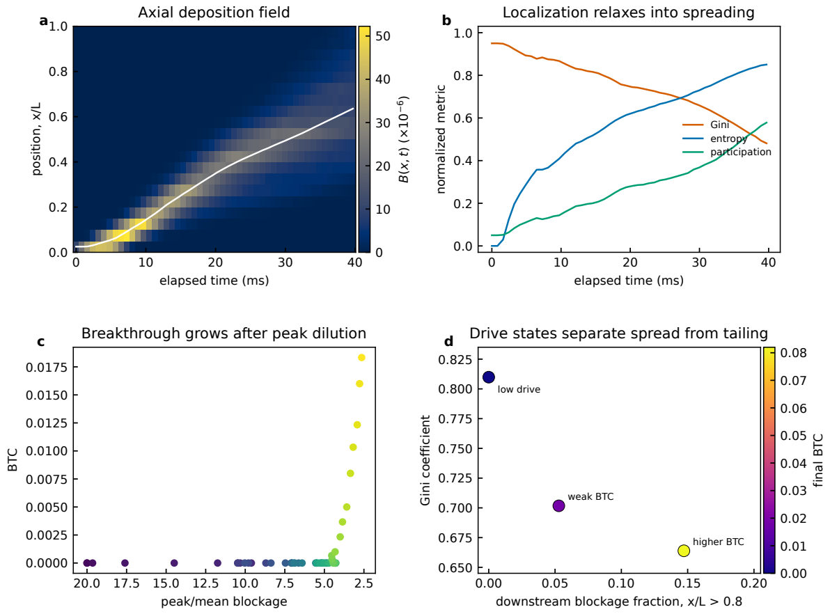
Fig. S8. spatial heterogeneity data mining of axial deposition profiles, localization relaxation and downstream spreading. Boundary: Spatial-deposition heterogeneity metrics derived from the axial blockage profiles.
