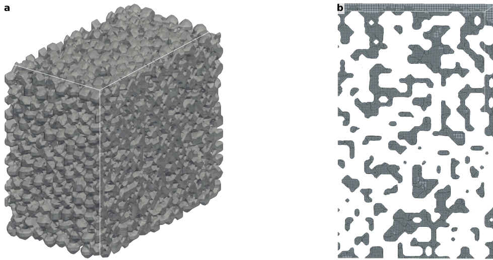
Fig. S7. ParaView-rendered OpenFOAM cropped-domain model and mesh slice. Boundary: Representative cropped-domain OpenFOAM geometry and mesh visualization.
