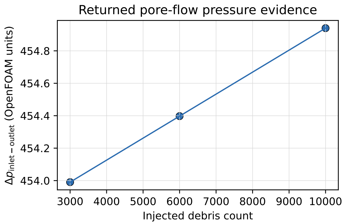
Fig. S6. returned cropped-domain OpenFOAM pressure evidence for peak-blockage handoff cases. Boundary: Cropped-domain OpenFOAM pressure-response check.
