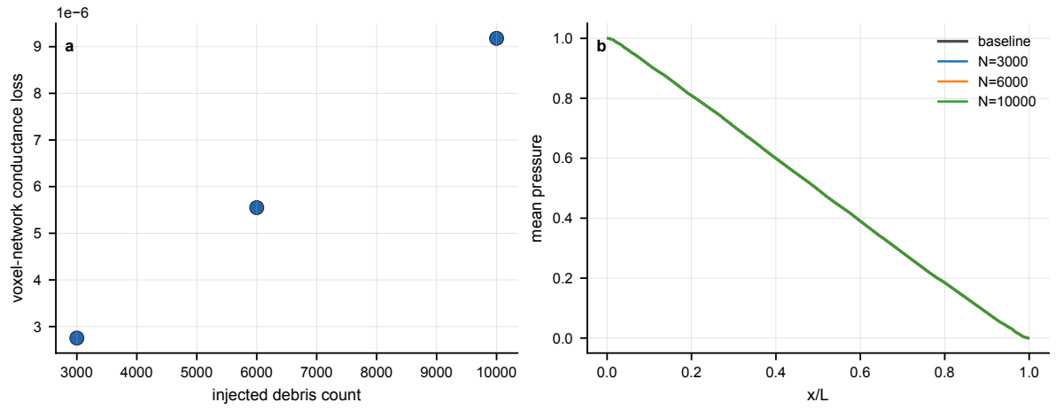
Fig. S3. voxel-network pressure pilot. Boundary: Scalar voxel-network pressure-response check.
