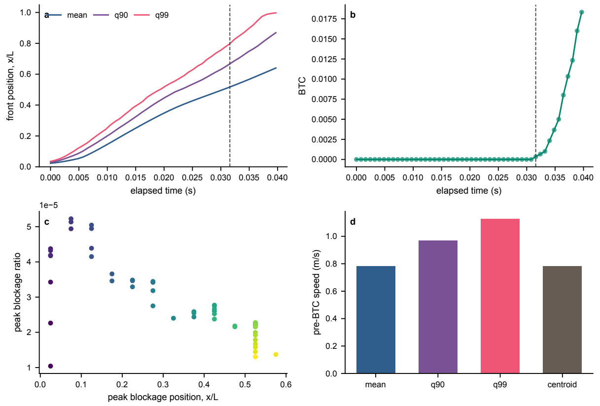
Fig. S2. front-migration speed fits. Boundary: Front-speed estimates for the representative drive case.
