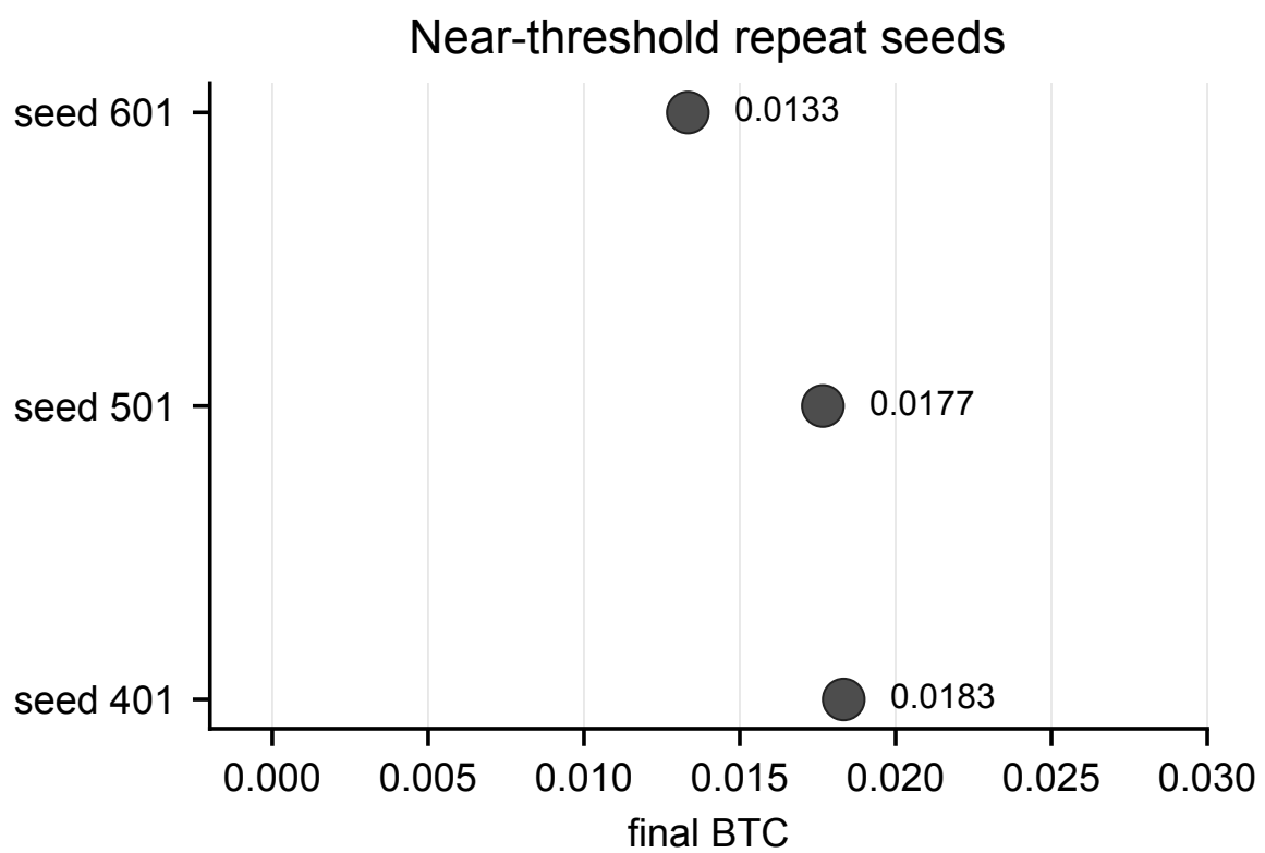
Fig. S5. near-threshold repeat-seed stochastic variability. Boundary: Repeat-seed variability for the near-threshold DEM setting.
