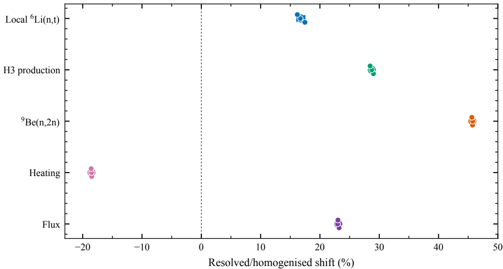
(a) PF = 0.618 independent hard-sphere realisations
