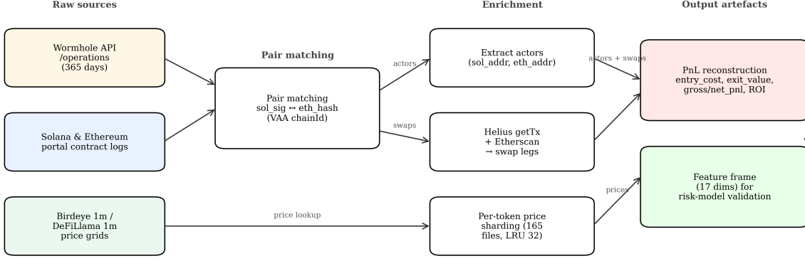
Figure 9 — Data-collection & processing pipeline for the 1-year Wormhole Portal study
