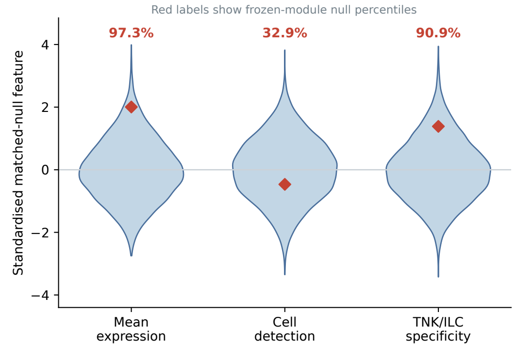
B Matching balance
