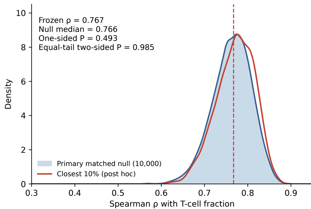
A Matched-null calibration in GSE178341
