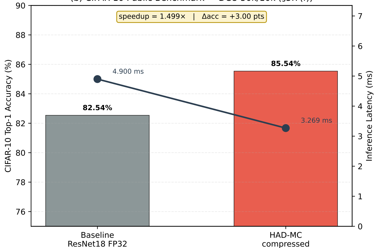
(b) CIFAR-10 Public Benchmark — DCU 50k/10k (§5.7(f))
