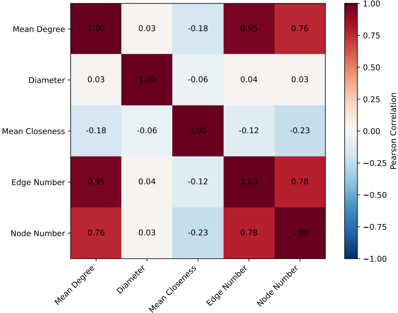
Network Metrics Correlation Matrix
