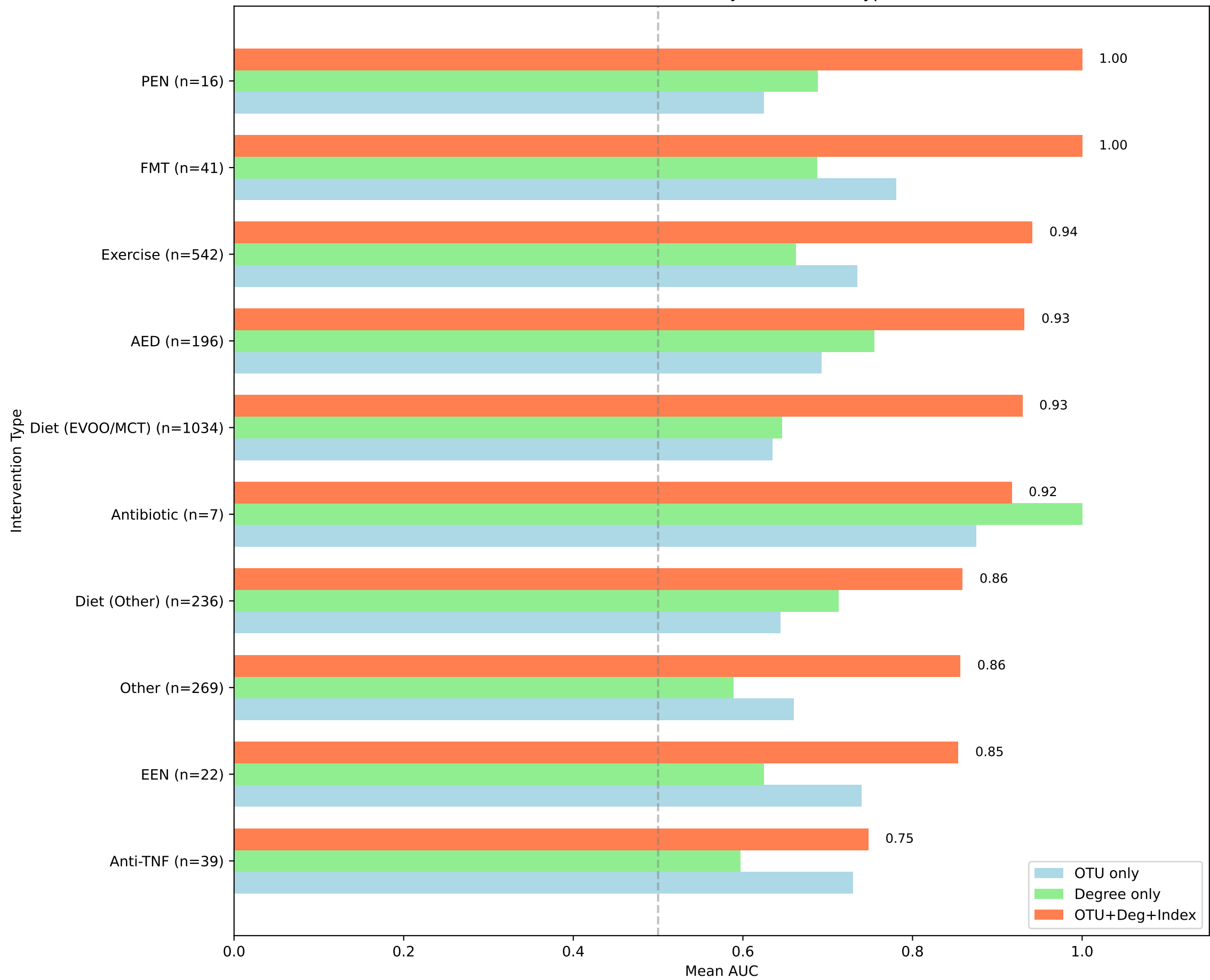
Model Performance by Intervention Type
